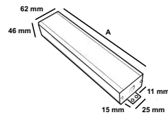
Product Drawing
